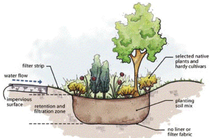
Bioretention cell
